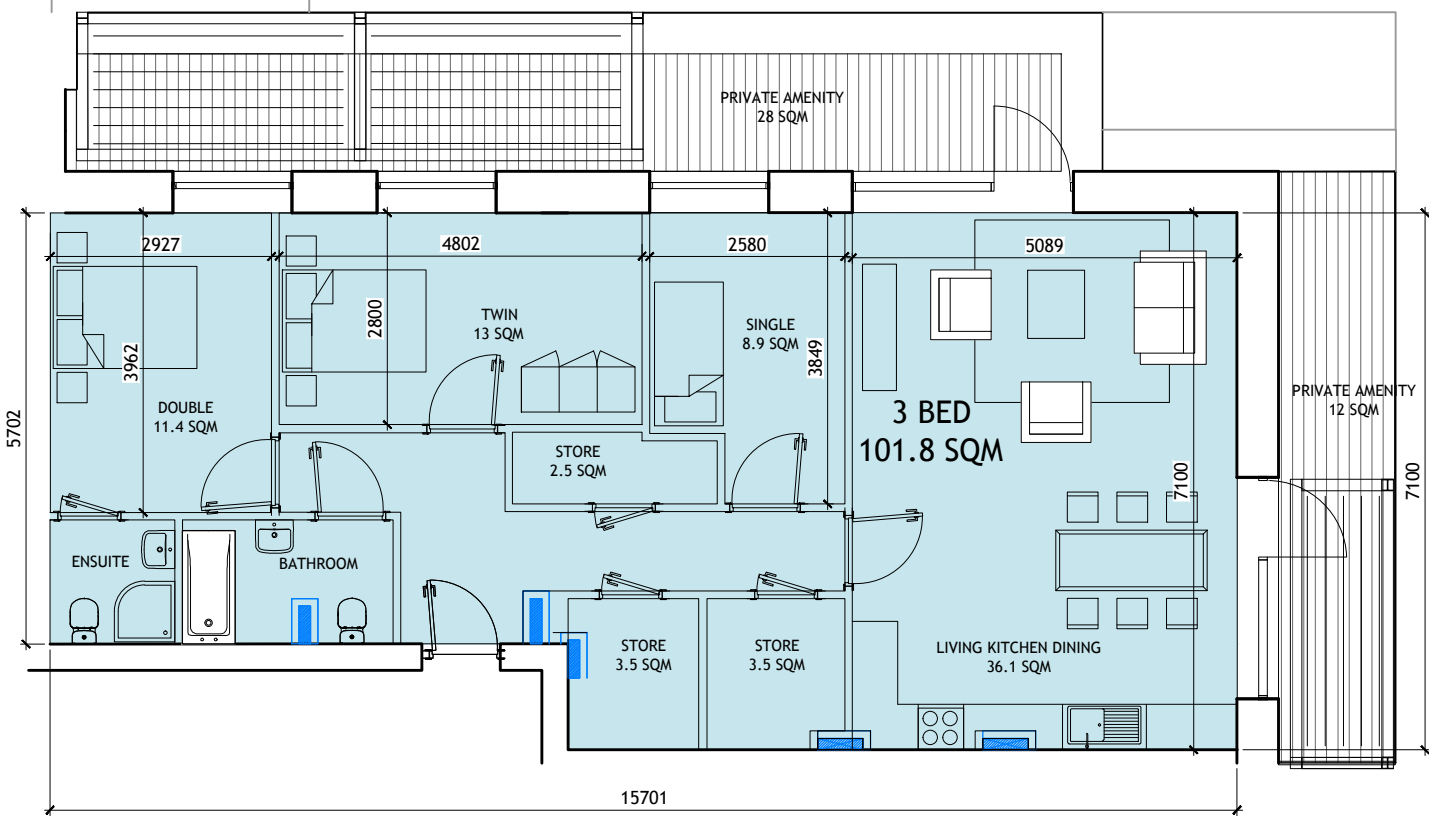
TYPE R (3 BED)
