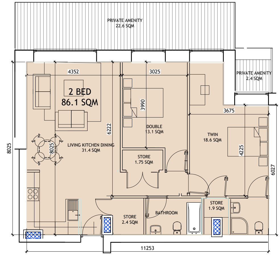
TYPE P (2 BED)
