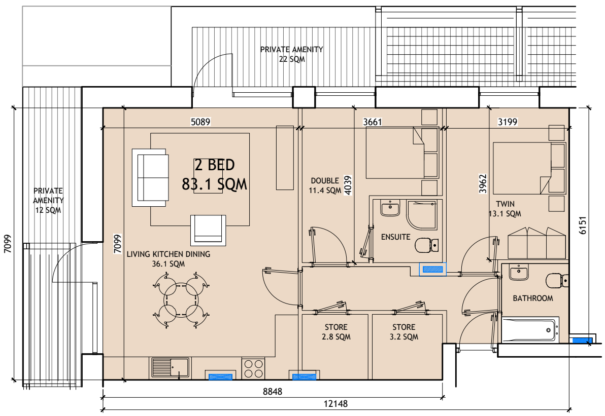
TYPE Q (2 BED)
